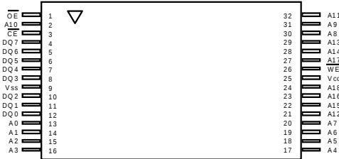
Reverse TSOP
