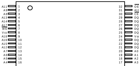
Standard TSOP
